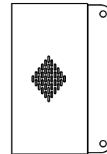
12" HEAT PANEL 48", 60" OR 72" LONG 1 TO 3 ELEMENTS
